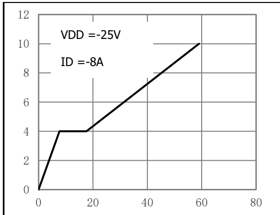
Fig.1 Gate-Charge Characteristics
