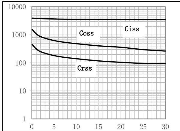
Fig.2 Capacitance Characteristics
